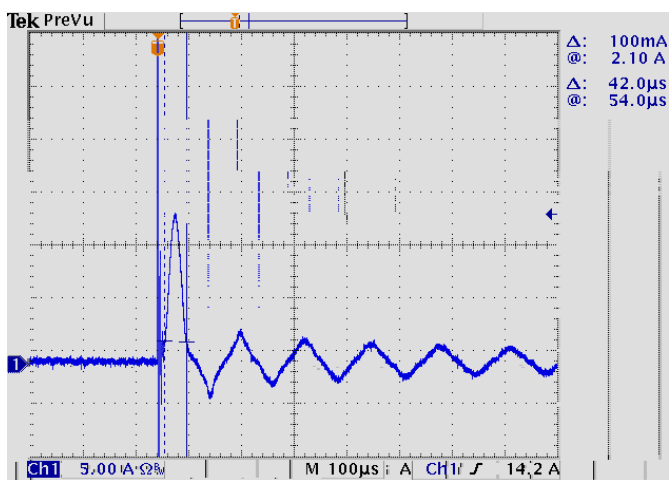
EDC-100S105ST( I_o=1050\text{mA} )
